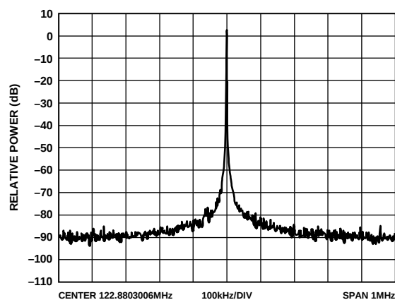
Figure 18. Output Spectrum, LVDS; 122.88 MHz; PFD = 15.36 MHz; LBW = 190 kHz; I_{CP} = 4.2 mA; F_{VCO} = 2.7 GHz
