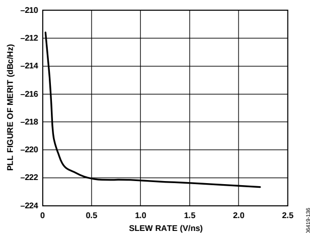
Figure 14. PLL Figure of Merit (FOM) vs. Slew Rate at REFIN/\overline{REFIN}
